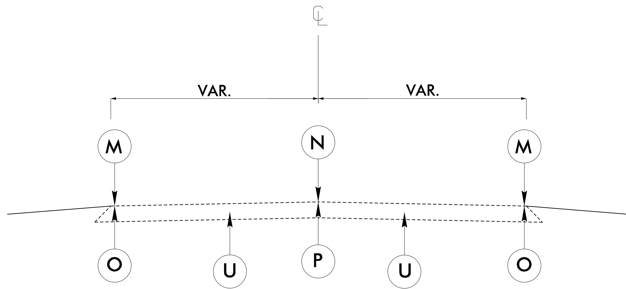
TYPICAL SECTION NO. 2 USE WITH MAPS: 2-8
