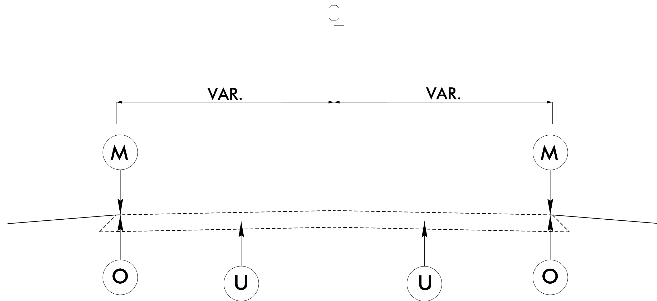
TYPICAL SECTION NO. 1 USE WITH MAP: 1
